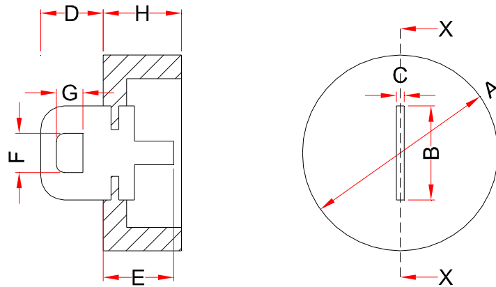
Section X-X
